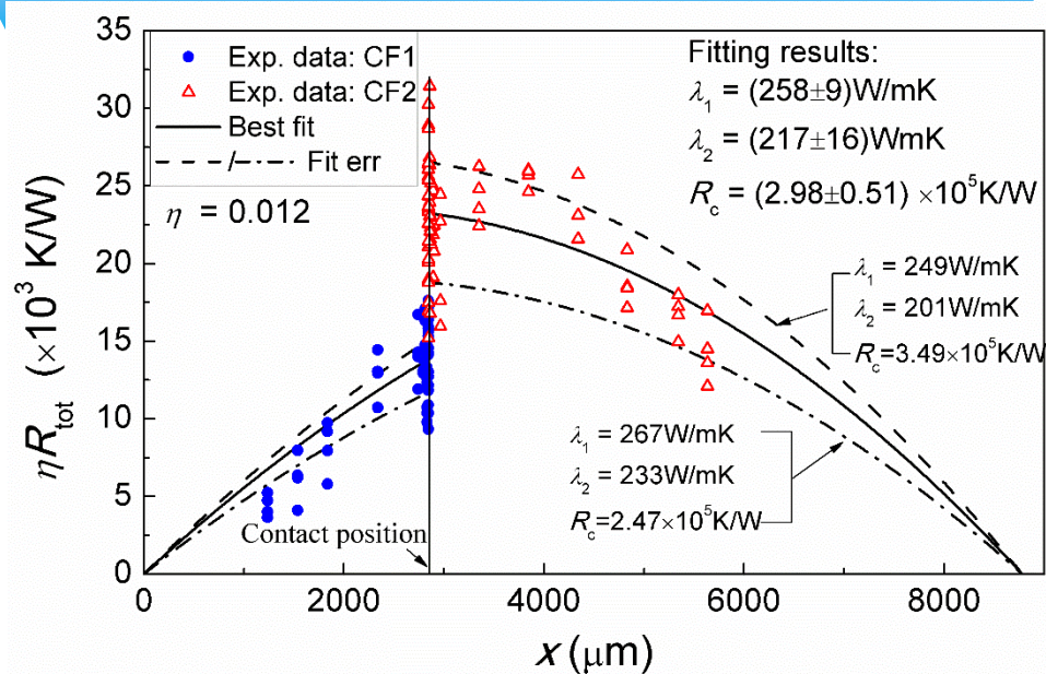
Absorptivity ( \eta ) measured by laser-flash Raman
