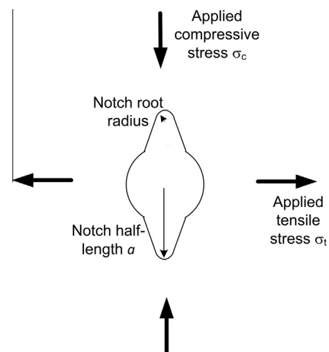
Fig. 1. Holes (of radius a ) were drilled into whole eggs. Some holes were extended by machining to produce sharp notches (of half-length a and root radius \rho ). Under an applied remote compressive load the local stress field in the vicinity of the hole/notch is biaxial, consisting of equal tensile and compressive stresses.
