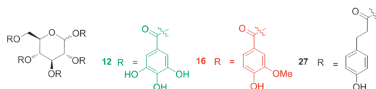
IC 50 of selected compounds against tumor cell
