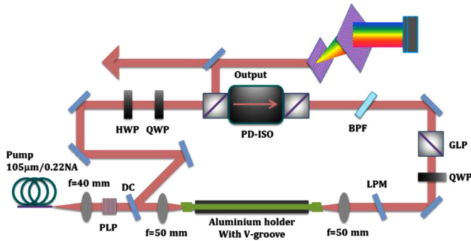
Fig. 1. Schematic diagram of the rod-fiber based ANDi laser. DM, dichroic mirror; PLP, pump laser protector; HWP (QWP), half- (quarter-) waveplate; PD-ISO, polarization-dependent isolator; BPF, birefringent plate filter; GLP, Glan laser polarizer; LPM, pump dump mirror. The rest unspecified mirrors are high reflective mirrors for the oscillated laser pulses in the ring cavity.
