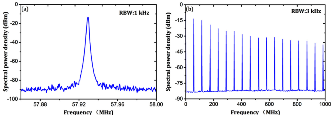
Fig. 3. RF spectra monitored with a photodiode and a frequency spectrum analyzer (Agilent E4407B). (a) The center repetition rate with 1 kHz resolution. (b) RF spectra with 1 GHz span.
