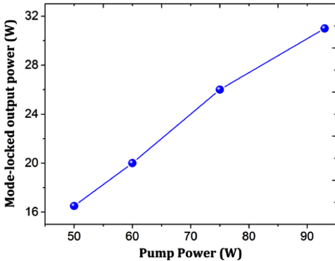
Fig. 2. Variation of the output power as a function of pump power.
