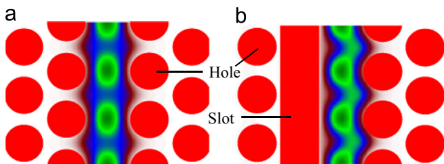
Fig. 2. Mode fields of the fundamental mode in (a) original and (b) slotted W1 PCW.
