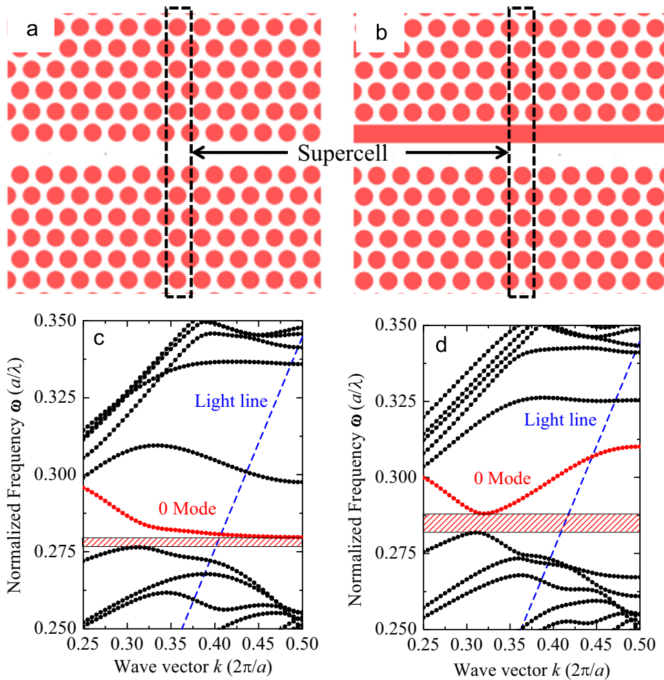
Fig. 1. Schematic of the (a) original and (b) slotted W1 PCW; (c) calculated dispersion curves of the original and (d) slotted W1 PCW. The dashed boxes present the supercells of the two PCWs. (For interpretation of the references to color in the text, the reader is referred to the web version of this article).
