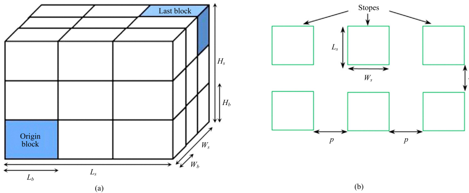
Fig. 2. An illustration of the stope and pillar layout notations.
