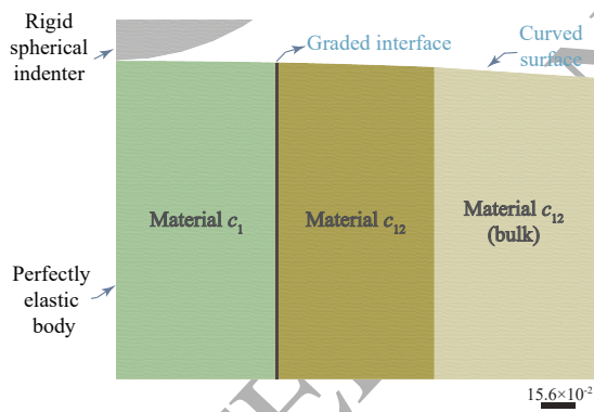
i) Axisymmetric contact region
