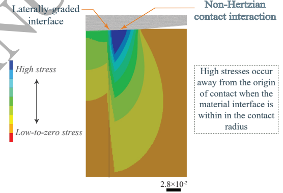
ii) Normal stress field
