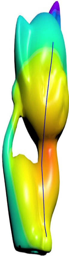
Open geodesic; Non-uniform density
