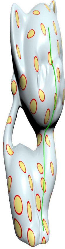
Open geodesic; Anisotropic metric
