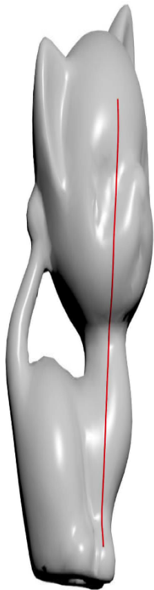
Open geodesic; Isotropic metric
