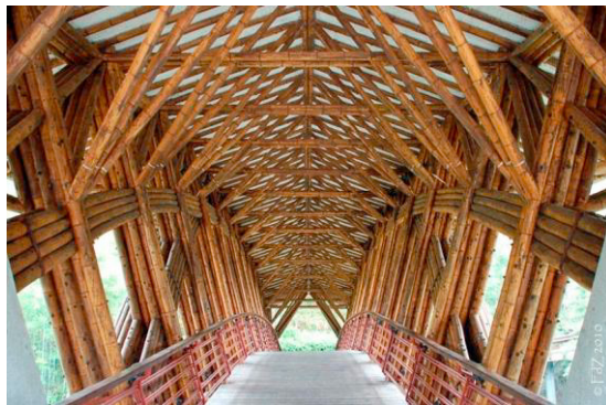
Fig. 2. Crosswaters Ecolodge's Bamboo Bridge, Guangzhou, China (2003). Simón Vélez. Adapted from [7].
