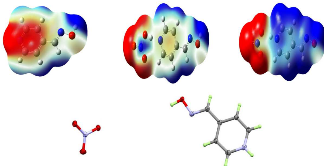
X-ray structure (lower) and MEP of P4A(left) and P4AN (gas, middle), (DMSO, right)
