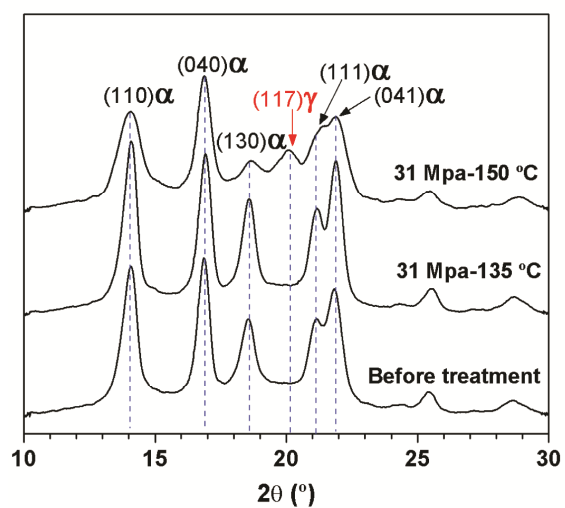
Isothermal annealing of PP/1.0 wt% CNT composites
