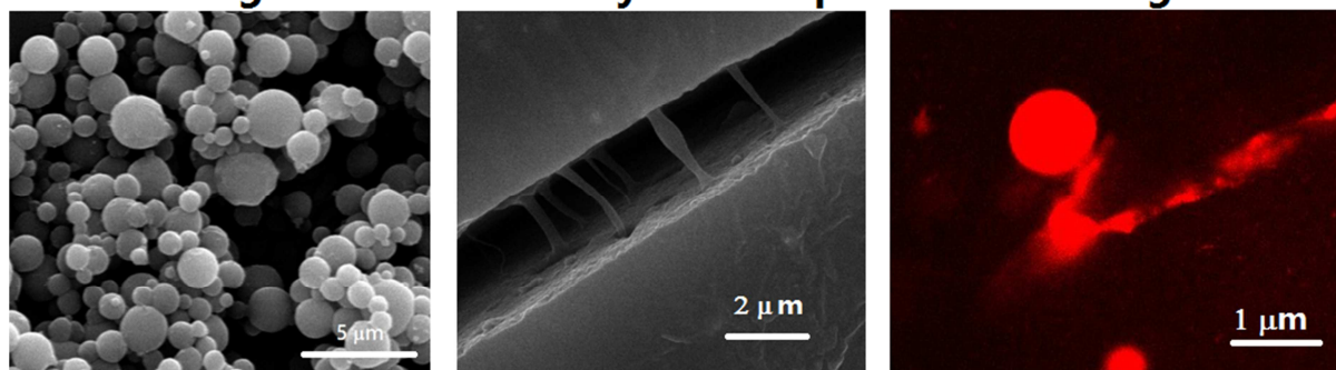
Self-healing of microcracks by microcapsules containing healant
