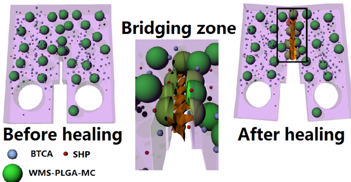
Self-healing of microcracks by microcapsules containing healant
