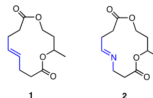
Figure 1. [13]-Macrodilide 1 and aza-[13]-macrodilide analog 2 .
