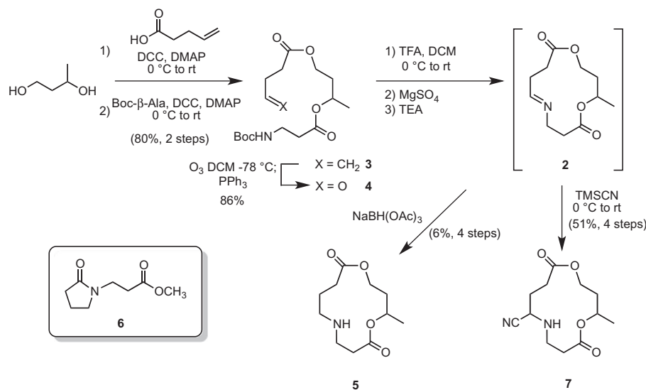
Scheme 1. Synthesis aza-[13]-macrodilolides 5 and 7 via macrocyclic imine 2 .
