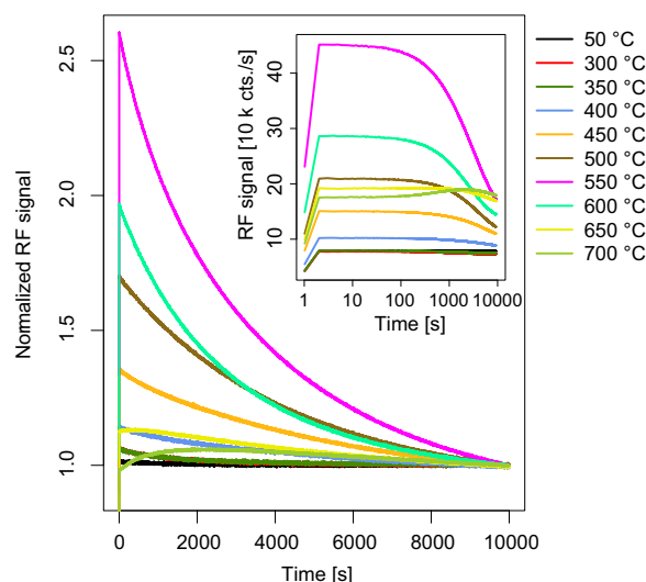
Fig. 1. UV-RF signal for sample BT586 for different preheat temperatures (hold for 120 s) prior to the RF measurements. For each temperature a new aliquot was used. The values are normalized to the last data point of each measurement and the total absorbed dose is 600 Gy during each RF measurement. For the sake of clarity the UV-RF curves for preheat temperatures from 100 °C to 250 °C were removed, because no change was observed. The inset shows the same data as the main figure but with absolute values and a logarithmic x-axis.
