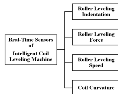
Fig. 3. Cyber-physical system of intelligent coil leveling machine
