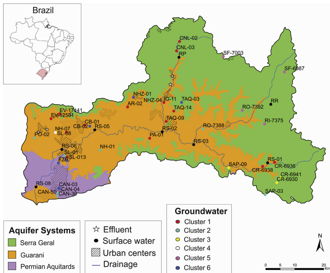
Fig. 1. RSW's hydrogeological map with sampling points and the groundwater clusters resulting from cluster analysis.
