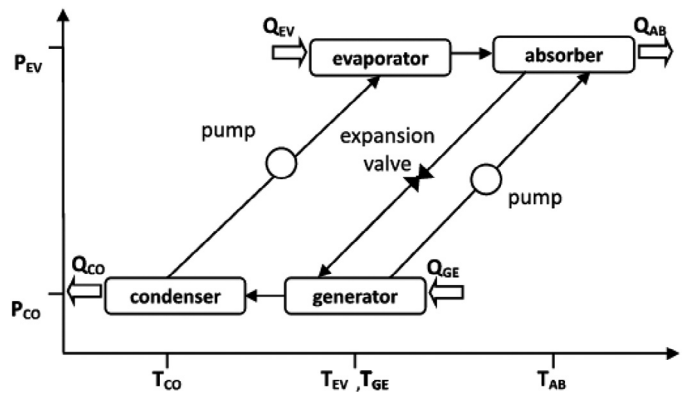
Fig. 1. Schematic diagram of a basic AHT.
