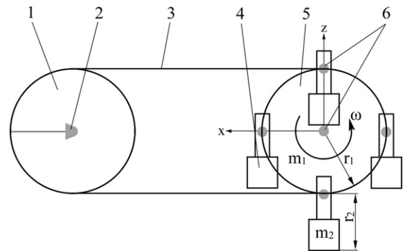
Fig. 1. MSC.visualnastran model of the hammer crusher. The hammers swing freely around the pivots fixed on the rotor. 1-pulley, 2-motor constraint, 3-belt constraint, 4-hammer, 5-rotor, 6-revolution joint constraint.
