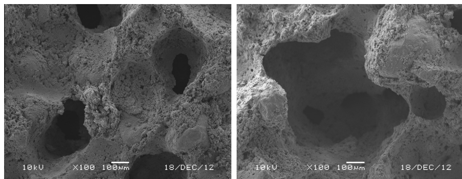
Fig. 1. SEM images of the structure of renovation plaster containing combined pores with different diameters.
