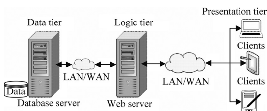
Fig. 1. Multiple-tier architecture as implemented by the webGC platform.
