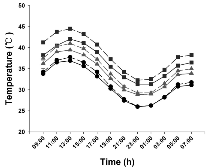
Fig. 2. The diel variation of ambient temperatures and body temperatures of Phrynocephalus przewalskii lizards under the three thermal treatments of 32 \pm 6^\circ\text{C} ( \circ ), 35 \pm 6^\circ\text{C} ( \blacktriangle ), and 38 \pm 6^\circ\text{C} ( \blacksquare ). — body temperature, ——— ambient temperature.
