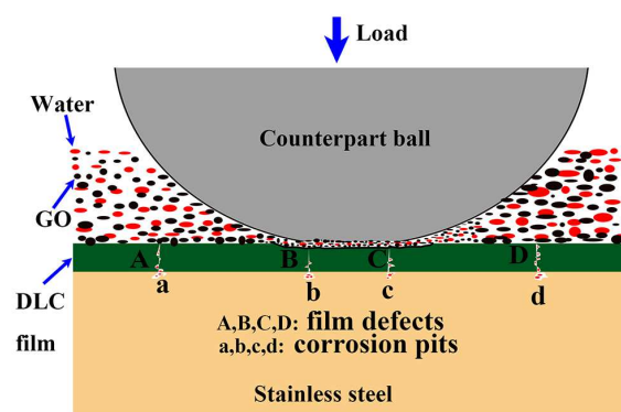
Tribocorrosion test
