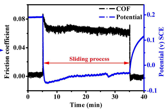
Typical OCP and COF curves
