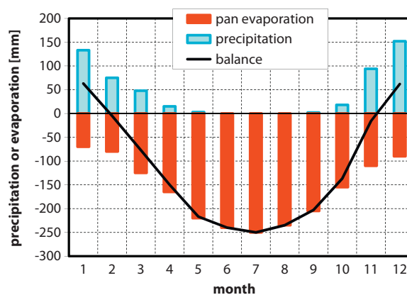
Fig. 1. Average monthly precipitation and pan evaporation for Tel Aviv. (Data: Bitan and Rubin [30]).
