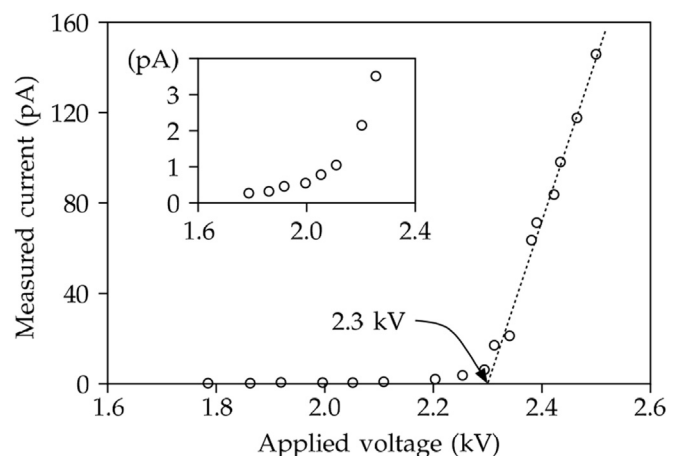
Fig. 4. Measured current with the electrometer as a function of the applied voltage to the wire.
