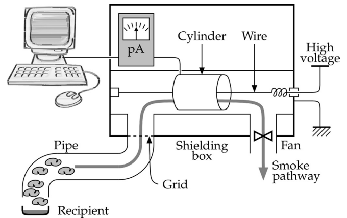
Fig. 3. Experimental set-up. The sensor prototype is placed in a Faraday shielding box. It is fed with smoke driven by a fan from a pipe.
