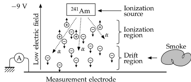
Fig. 2. Principle of an ionic smoke sensor. In presence of smoke, much less charged particles reach the measurement electrode.
