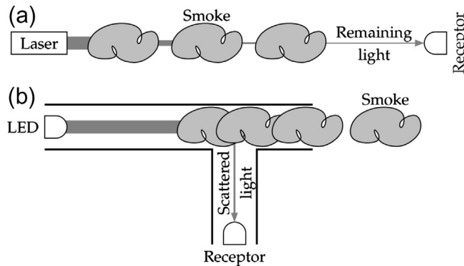
Fig. 1. Principle of optical smoke sensors. (a) Operating mode for a detection over large areas. (b) Operating mode for a punctual detection. The source is often a light emitting diode (LED).
