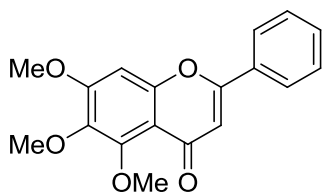
5,6,7-trimethoxyflavone, 2
