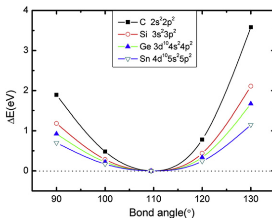
Fig. 2. Energy change via bond angle distortion from 109.471^\circ to 90^\circ , 100^\circ , 120^\circ and 130^\circ .
