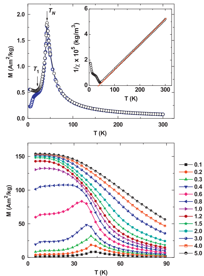
Fig. 1. Temperature dependences of zero-field-cooling (ZFC) and field-cooling (FC) magnetizations for TbPdAl in a magnetic field of 0.05 T. The inset shows the reciprocal magnetic susceptibility \chi^{-1} versus temperature in a field of 0.05 T.
