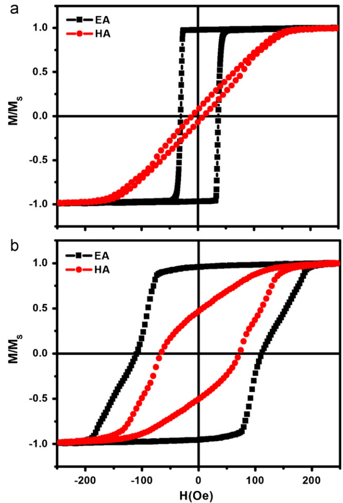
Fig. 2. In-plane hysteresis loops of (a) x=9 nm film and (b) x=96 nm film. (EA is parallel to easy axis of uniaxial anisotropy, and HA is hard axis).
