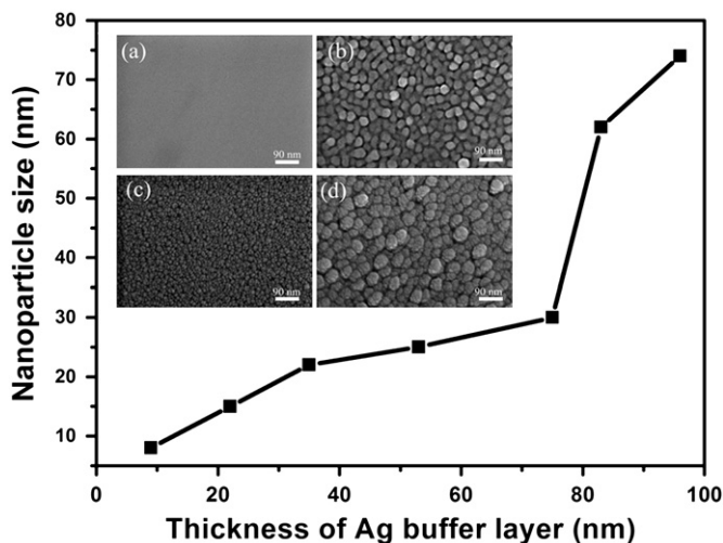
Fig. 1. The variation of nanoparticle size as a function of Ag buffer layer thickness. Insets are SEM images of single Ag film of (a) 9 nm, (b) 75 nm, and (c), (d) SEM images of as-deposited \text{Co}_{92}\text{Zr}_8(50\text{ nm})/\text{Ag}(x) films for x=9 nm x=75 nm.
