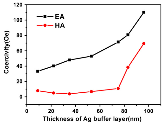
Fig. 3. Coercivity H_c of \text{Co}_{92}\text{Zr}_8(50\text{ nm})/\text{Ag}(x) films as functions of Ag buffer layer thickness.
