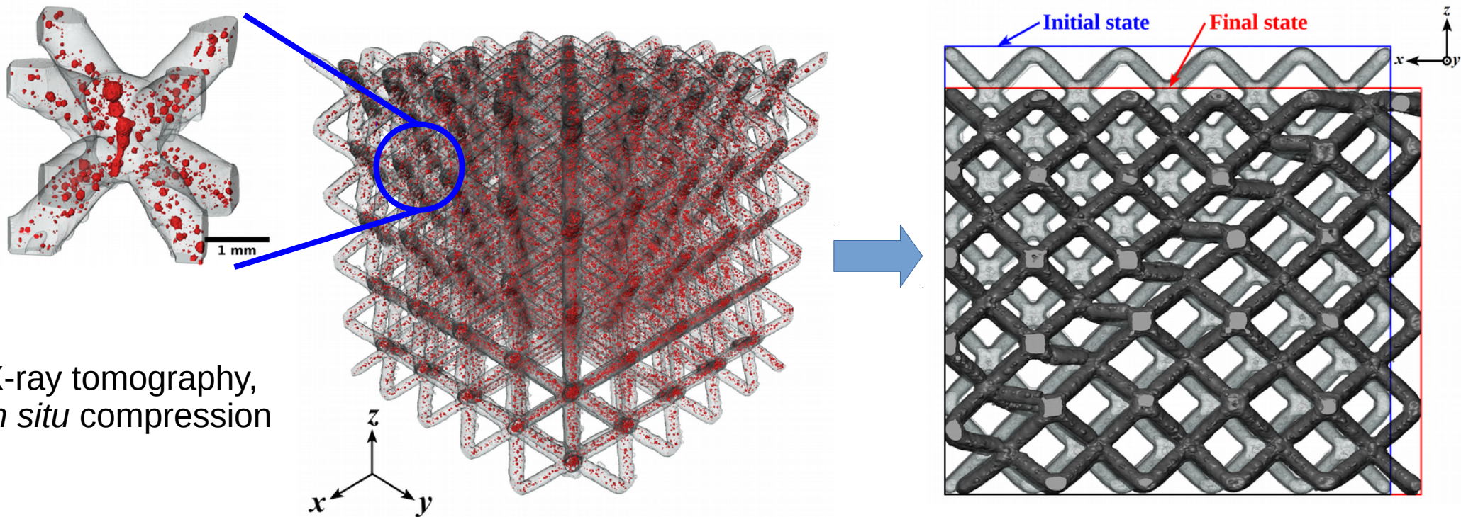
Finite element analysis, image-based 3D mesh
