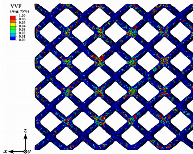
Finite element analysis, image-based 3D mesh
