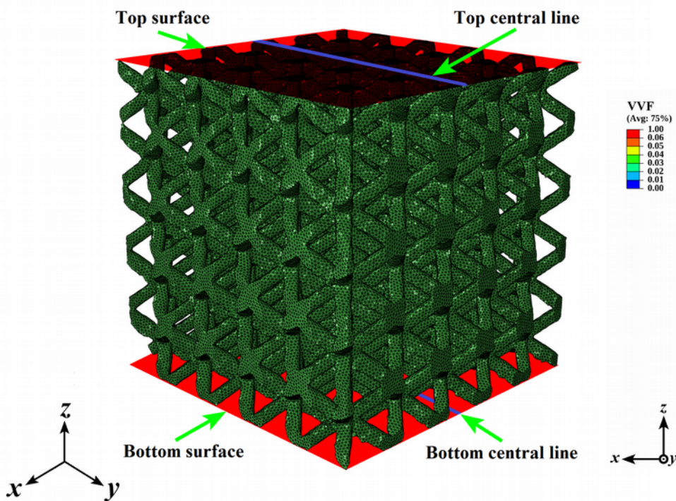
Finite element analysis, image-based 3D mesh
