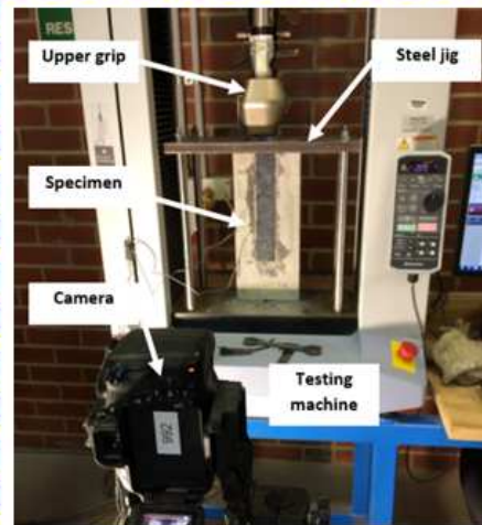
Testing setup
