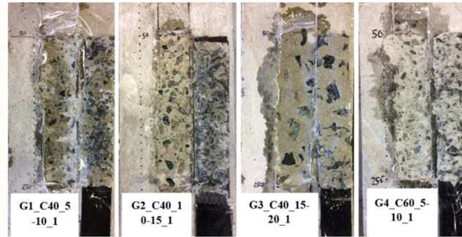
Specimens (Different aggregate sizes)
