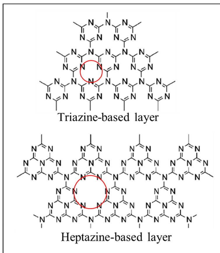
Postulated planar \text{C}_3\text{N}_4 extended structures ( \text{g-C}_3\text{N}_4 )
