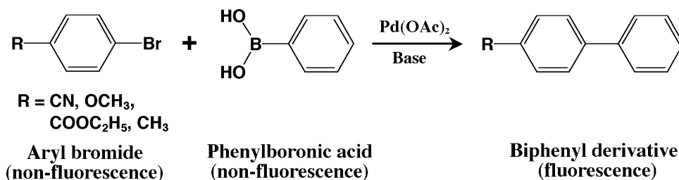
Fig. 1. Scheme of the proposed fluorogenic derivatization reaction for aryl bromide.
