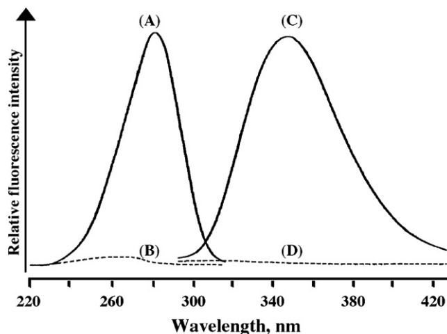
Fig. 2. Fluorescence spectra obtained from the reaction mixture of BrPhCOOC 2 H 5 with PBA and the reagent blank. Excitation spectra with the emission wavelength at 350 nm of the product (A, solid line) and the reagent blank (B, dashed line). Emission spectra with the excitation wavelength at 290 nm of the product (C, solid line) and the reagent blank (D, dashed line).
