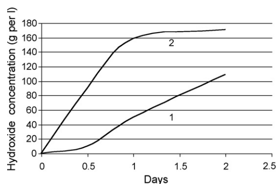
Fig. 2. Diffusion of \text{OH}^- ions through separator F and M (1) microporous separator; (2) rayon-type separator.
