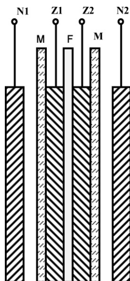
Fig. 1. Setup 1 N1 and N2: nickel oxide electrodes; Z1 and Z2: zinc electrodes; M: microporous separators; F: rayon-type separator.
