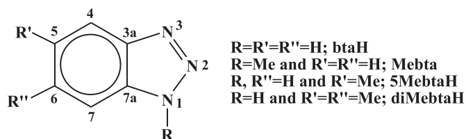
Scheme 1. The general structural formula of benzotriazoles. The parent member of this family of ligands is 1H-benzo[d][1,2,3]triazole or simply benzotriazole (btaH; R=R'=R''=H ). R, R' and R'' can be non-donor (Me, Cl, \text{NO}_2 ,...) or donor (OH, COOH, \text{CH}_2\text{OH} , \text{CH}_2\text{COOH} ,...) groups. The ligands used and discussed in this work are 1-methylbenzotriazole (Mebta; R=\text{Me} , R'=R''=H ), 5-methylbenzotriazole (5MebtaH; R=\text{Me} , R=R''=H ) and 5,6-dimethylbenzotriazole (diMebtaH; R'=R''=\text{Me} ; R=H ).
