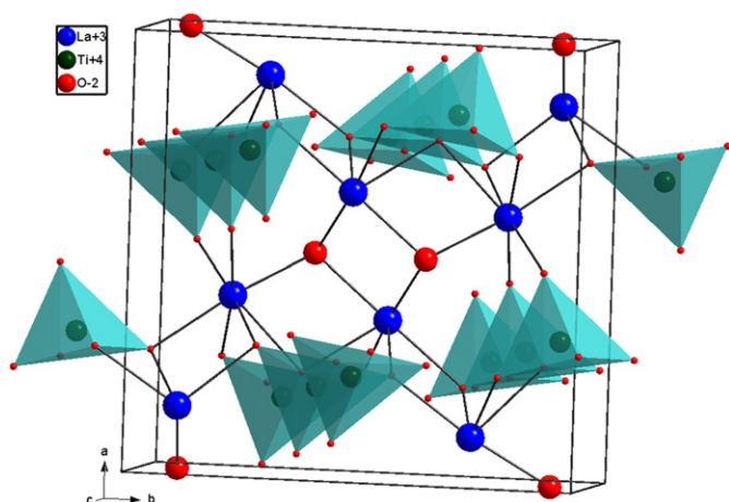
Fig. 1. Schematic crystal structure of orthorhombic \text{La}_2\text{TiO}_5 with space group Pnam (ICSD #28277).
