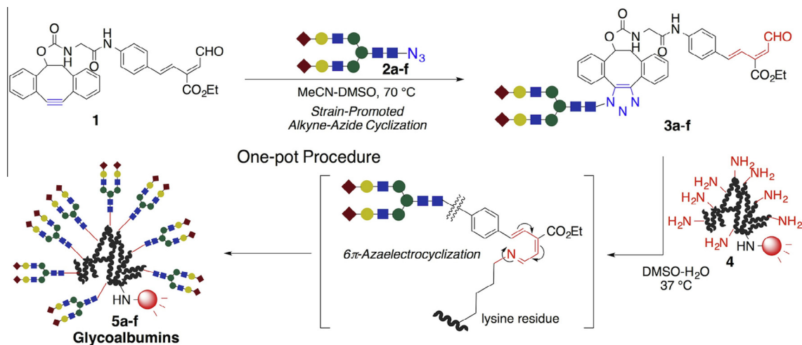
Figure 1. One-pot preparation of the glycoalbumins 5a–f via strain-promoted alkyne-azide cycloaddition and 6\pi -azaelectrocyclization. 21
