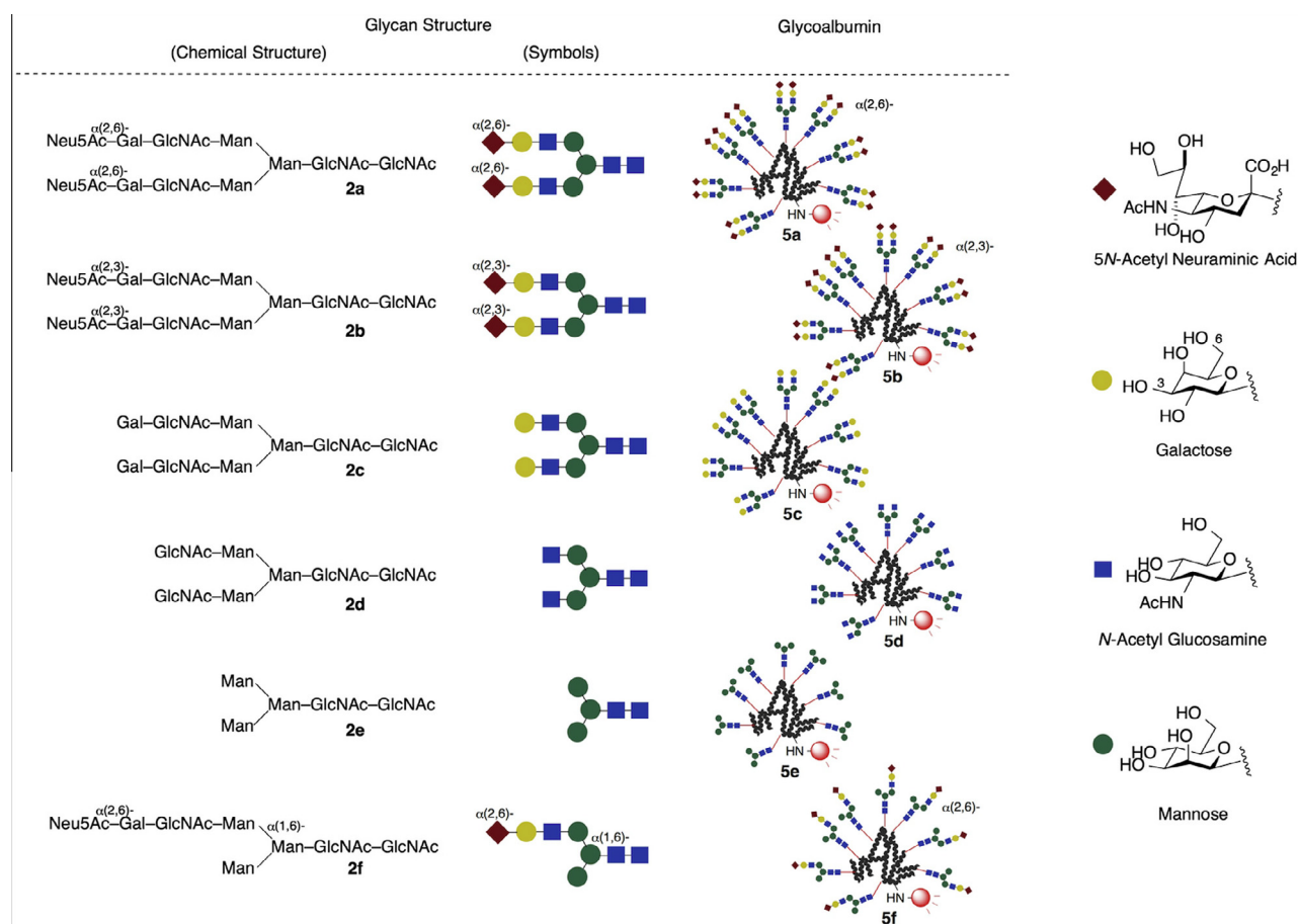
Figure 2. Structures of the N -glycoclusters 5a–f examined in this research.
