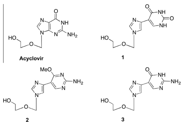
Figure 1. Acyclovir (ACV) and target fleximer analogues (1–3).
