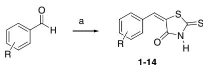
Scheme 1. Reagents and condition: (a) 2-Thioxo-thiazolidin-4-one, \beta -alanine, AcOH, reflux.
