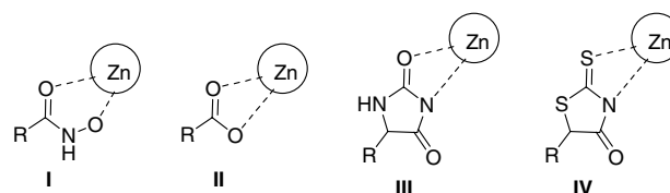
Figure 1. Zinc binding modes associated with various known bidentate zinc chelators: (I) hydroxamic acid, (II) carboxylic acid, (III) hydantoin, and (IV) thioxothiazolidinone.
