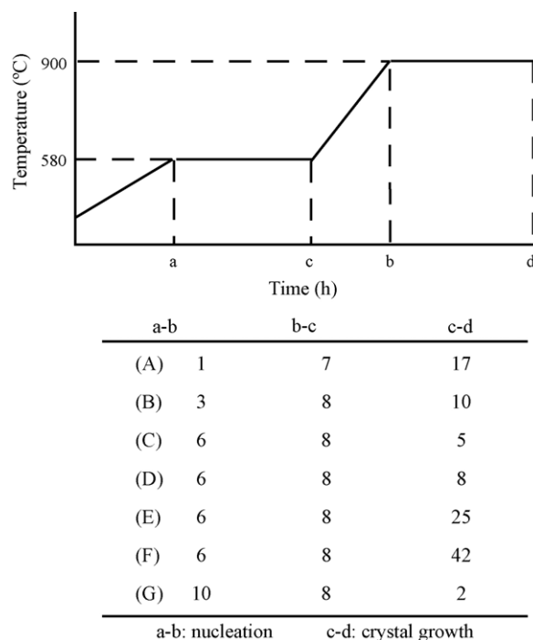
Fig. 1. The programs of temperature and time for the production of glass-ceramics.
