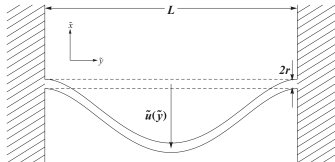
Fig. 1. Schematic representation of a doubly clamped nanomechanical resonator of the length L and the radius r . An applied force induces the bending profile \tilde{u}(\tilde{y}) as indicated.
