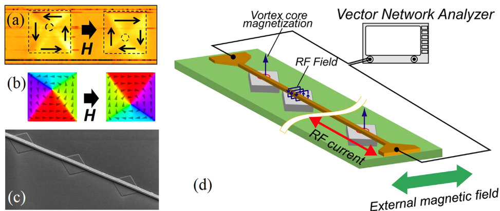
Fig. 1. (a) Spatial distribution of the spin structure in the squared Permalloy dot observed by magnetic-force microscope; (b) numerically simulated vortex structures stabilized in squared dot under the external field parallel to the edge; (c) SEM image of part of the fabricated device; (d) schematic illustration of the sample structure together with the SEM image of the fabricated sample.
