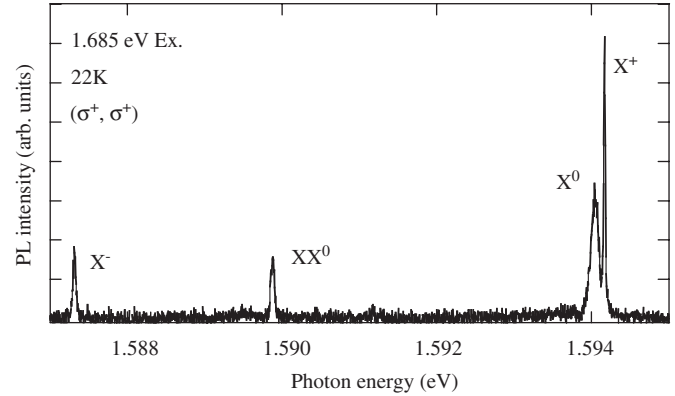
Fig. 1. High-resolution PL spectrum from an InAlAs single QD. Positively charged exciton ( X^+ ), neutral exciton ( X^0 ), neutral biexciton ( XX^0 ), and negatively charged exciton ( X^- ) dominate the spectrum.
