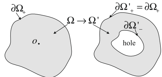
Fig. 1. Transformation from the region \Omega to \Omega' for constructing a perfect cloak. The outer boundary \partial\Omega_+ of the region \Omega is kept unchanged, and the point \mathbf{O} inside of \Omega is transformed to the inner boundary \partial\Omega'_- of \Omega' . Except a point \mathbf{O} and \partial\Omega'_- , the transformation is everywhere one-to-one and differentiable.
