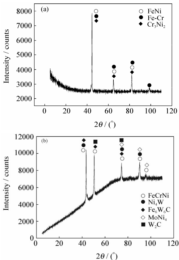
Fig. 3. XRD patterns of the substrate (a) and the laser alloying layer (b).
