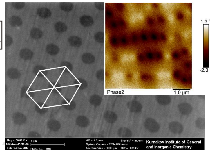
SEM and MFM images
