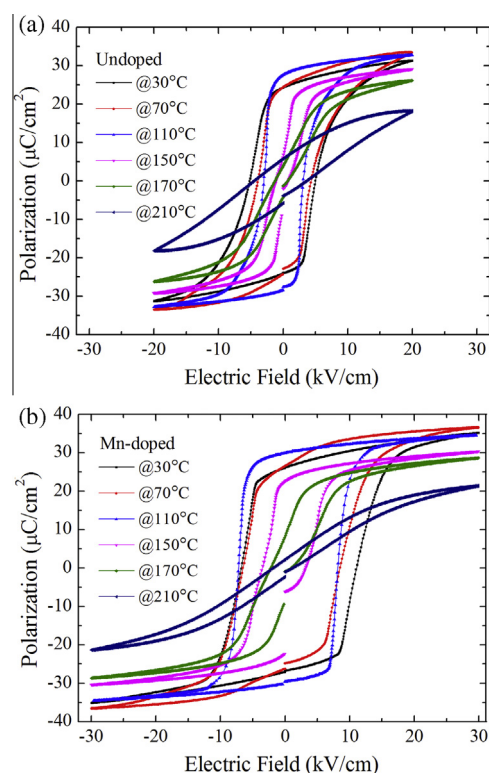
Fig. 1. Temperature dependence of P – E hysteresis loops in (a) undoped and (b) Mn-doped [001]_c -oriented 0.24PIN–0.47PMN–0.29PT single crystals.
