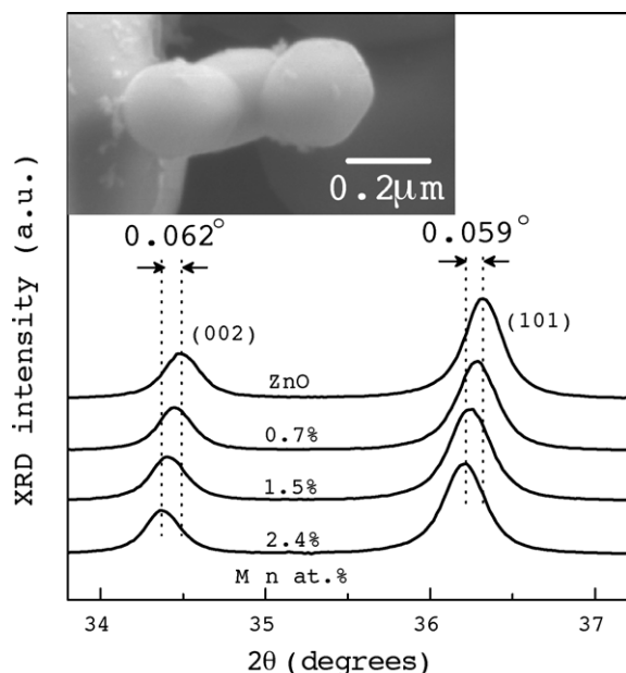
Fig. 1. XRD of pure and Mn-doped ZnO nanoparticles. Peak shifts of 0.059^\circ and 0.062^\circ were observed for the (101) and (002) lines of 2.4 at% Mn-doped ZnO with respect to pure ZnO. The inset shows an SEM image of ZnO nanoparticles.
