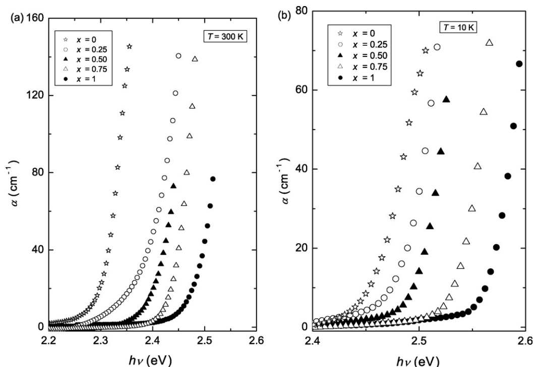
Fig. 1. Absorption coefficients vs. photon energies for \text{TlGa}_x\text{In}_{1-x}\text{S}_2 mixed crystals at T = 300\text{ K} (a) and T = 10\text{ K} (b).
