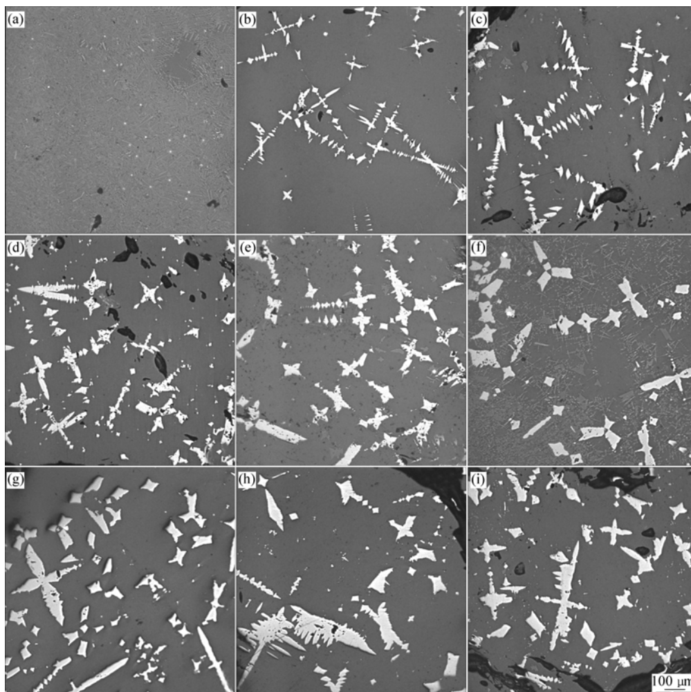
Fig.1 Micrographs of samples of slag heated at 1 593 K for 5 min (a); 10 min (b); 15 min (c); 20 min (d); 30 min (e); 50 min (f); 70 min (g); 90 min (h) and 110 min (i)
