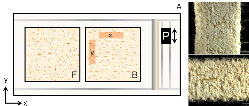
Fig. 1. Schematic top view of 3D printing (A). Feed chamber (F) and build chamber (B) are localized in x - y plane. Samples are labelled with x and y according to their orientation in the building chamber. The print head (P) moves across the building chamber in x direction where binder is sprayed in y direction (see arrow next to P). Figure B ( y orientation) and C ( x orientation) shows predominant fibre orientation within the samples.
